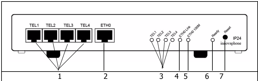
Fig. 1 - Indicators and connectors of the IP24
