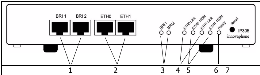
Fig. 1 - Indicators and connectors of the IP305
